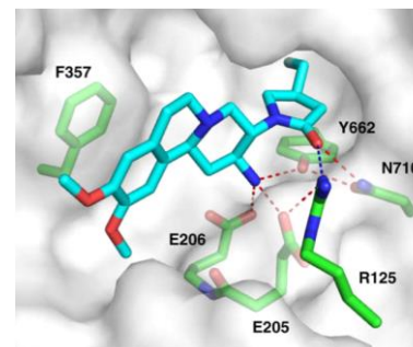
Crystal structure of DPP-IV with Carmegliptin
