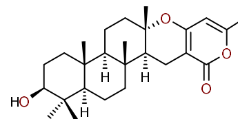
Chevalone A
