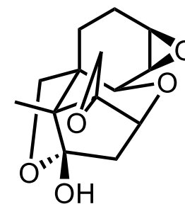
4,11-diepi-12,13-deoxyverrucarol
